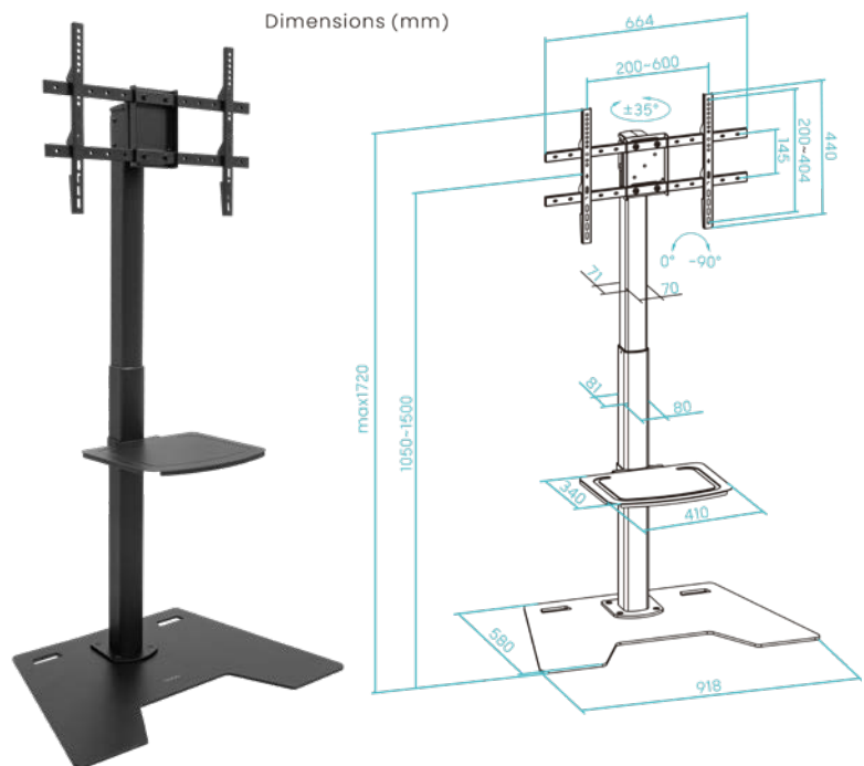
Dimensions (mm)
